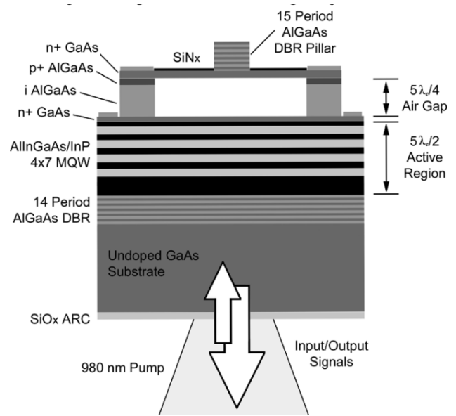
Fig. 1. Cross-sectional schematic of the bottom-emitting tunable VC SOA.
