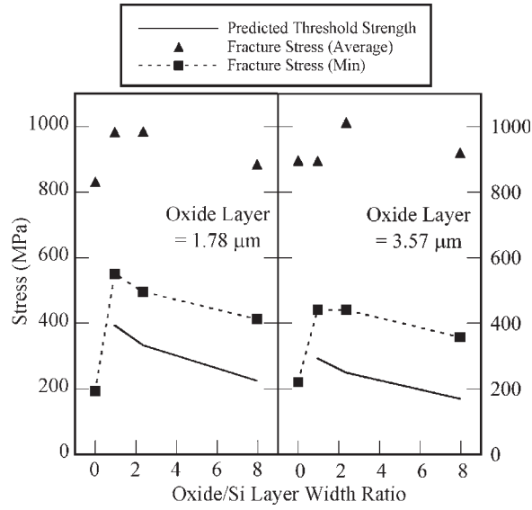
Figure 2. Fracture testing results from [3] for silicon–silicon oxide composites for MEMS applications. The minimum fracture strength for the composites is significantly higher than the minimum fracture strength for the monolithic silicon structures.
