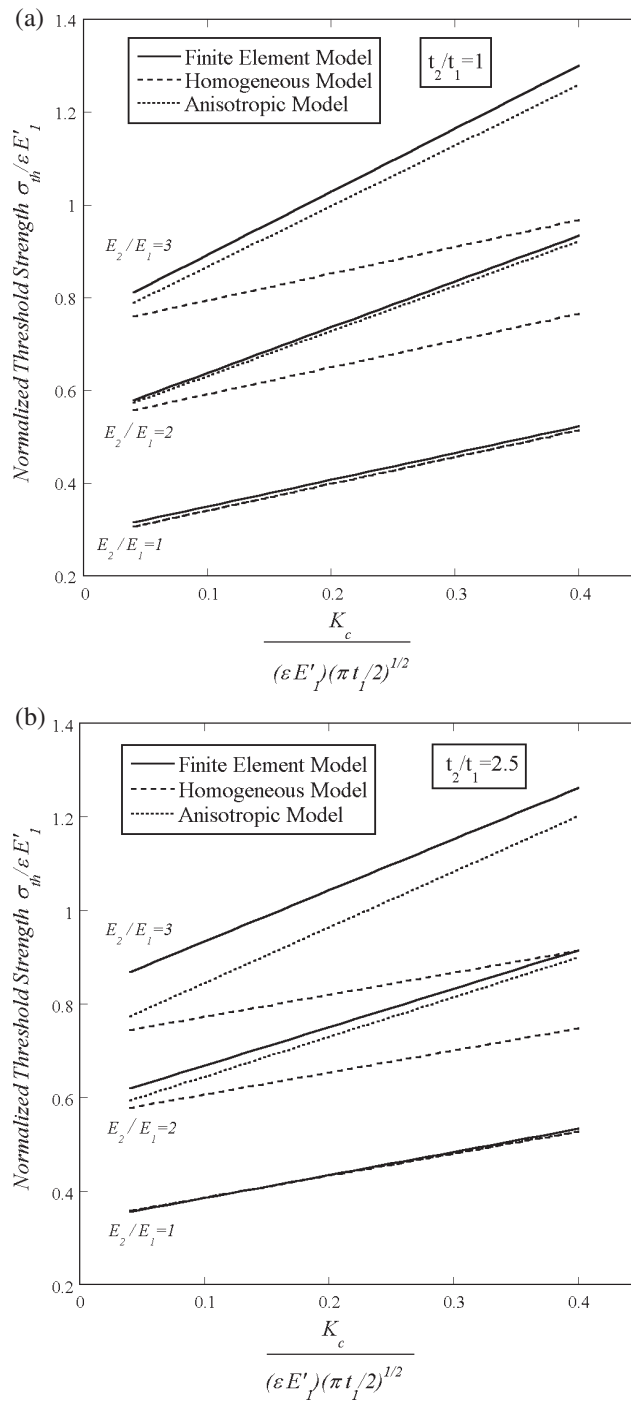
Figure 5. A comparison of the predictions from the homogeneous analytical model, the finite element simulations and the anisotropic model for the threshold strength versus normalized fracture toughness at various ratios of material modulus and layer widths.
