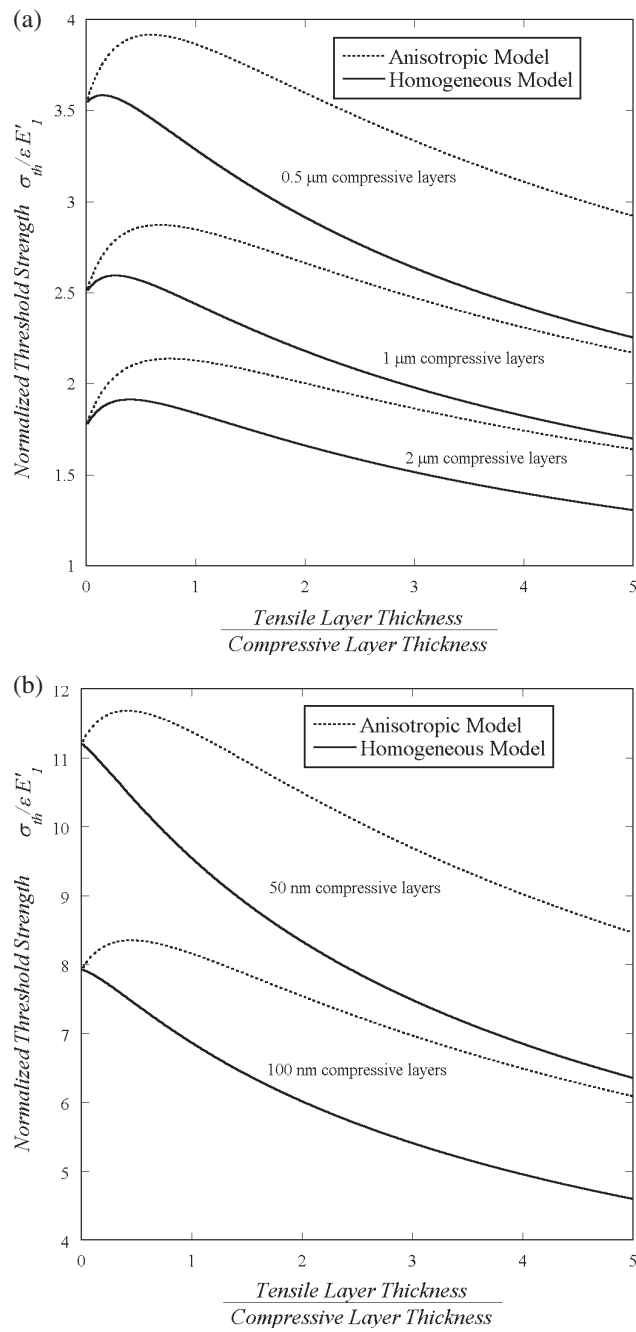
Figure 6. Variation of the normalized threshold strength with layer width ratio at different size scale of layer widths. Comparative results from both analytical models are presented.
