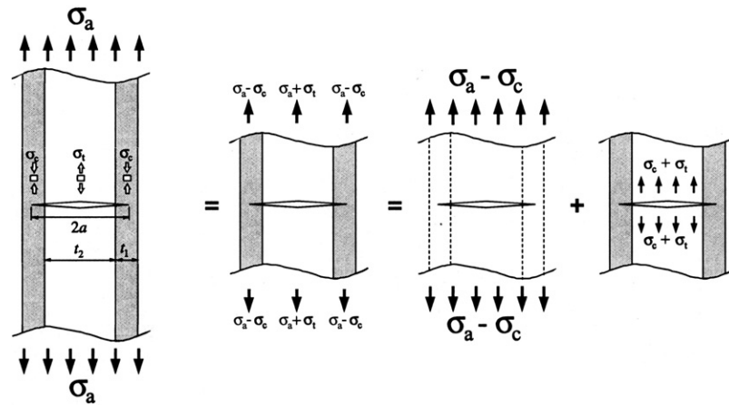
Figure 3. A schematic of the crack geometry and residual and applied stresses assumed in the mathematical modelling. The crack is assumed to just extend into the compressive layers. The stress superposition scheme used to obtain the crack tip stress intensity factor is also indicated here.
