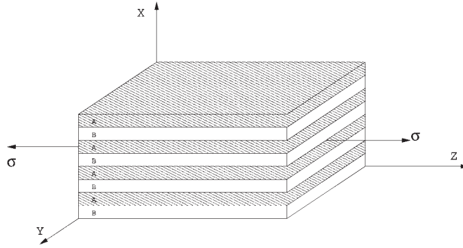
Figure 4. A schematic of the bimaterial laminate geometry; 2-3 is the plane of transverse isotropy for this model. The elastic problem is solved for a uniform stress applied one by one along the x , y , and z axes to obtain the compliance matrix.
