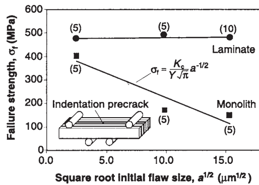
Figure 1. Fracture testing results on an alumina–mullite laminate [1]. The fracture strength is seen to be independent of initial crack size for the composite, but inversely related to crack size for the monolithic ceramic structures. Reprinted with permission from Rao M P et al 1999 Science 286 102–5. © 1999 AAAS.
