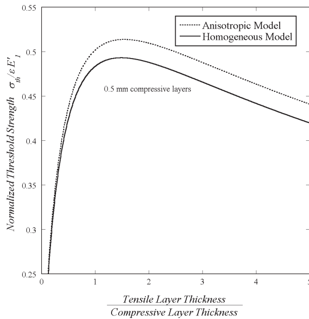
Figure 7. Variation of the normalized threshold strength with layer width ratio at millimetre scale layer widths. Comparative results from both analytical models show little variation at these size scales.
