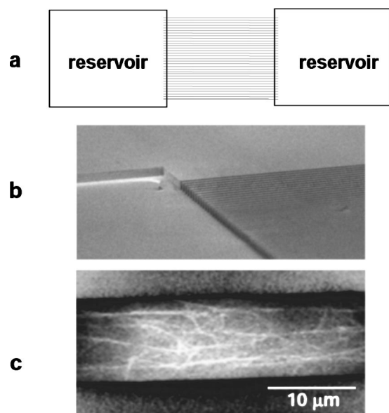
FIG. 2. (a) Schematic layout of the microchannel device; (b) SEM image of a section of the device; (c) fluorescence micrograph of 0.1 mg/ml actin bundled with 0.1 mg/ml \alpha -actinin inside a single 10- \mu m-wide \times 10- \mu m-deep-channel. The bundles are predominantly aligned parallel to the channel.
