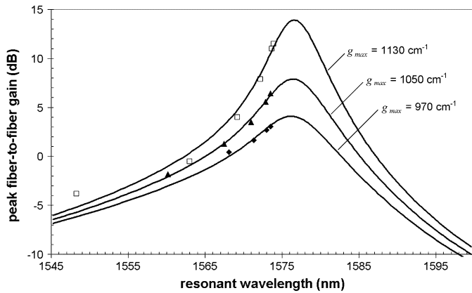
Fig. 12. Theoretical and experimentally measured peak fiber-coupled gain as a function of the resonant cavity wavelength of the VCSCOA. The theoretical curves are generated from (16), after matching the wavelength tuning response in (15).
