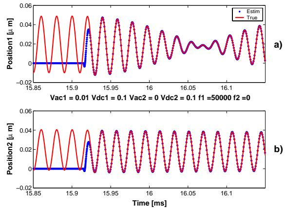
Fig. 6. Steady state oscillation of Cantilever 1 (a) and Cantilever 2 (b) and detail of the transient when the controller is switched on. The solid line is the cantilever oscillation, the dotted line its estimate. Notice the fast transient of the observer.
