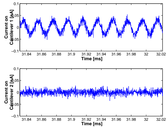
Fig. 10. Simulation of sensor noise : current measured on both cantilevers.
