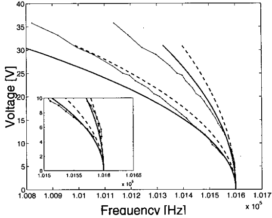
Fig. 2. The thin line (overlying the dots) is an experimentally determined map of the first parametric resonance region in the microcantilever. The dotted line shows the analytical result, using the Q and natural frequency determined from experiment, and the solid line shows the analytical result when using Q and natural frequency and electrostatic stiffness determined from experiment.
