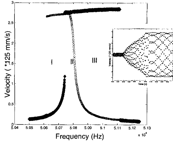
Fig. 5. Combined harmonic/parametric frequency response. Note that there are bistable regions (I and III) on either side of the parametric tongue (II).
