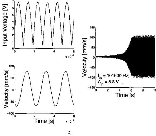
Fig. 3. Time series of a typical input and output inside the first 'tongue'. Note the response is at half the driving frequency.
