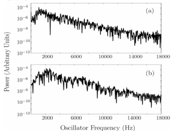
Fig. 4 Broadband power spectrum of a chaotic attractor found (a) experimentally and (b) numerically for the same parameters as Figure 3 (the velocity units prior to taking the Fourier transform are identical to Figure 3 (a) and (b)).
