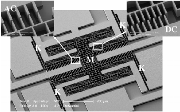
Fig.1 SEM image of the chaotic oscillator.
